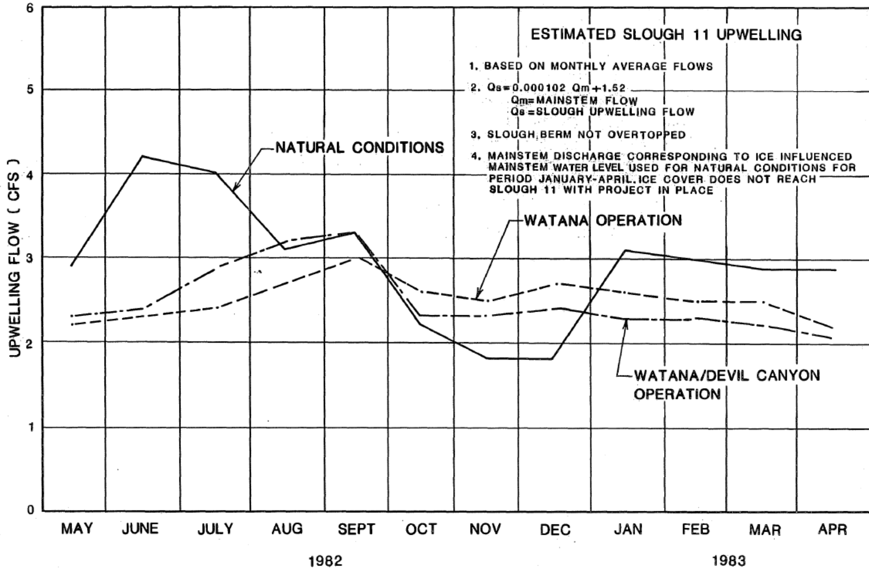
Figure 12. Estimated Slough 11 Upwelling Under Natural and With-Project Conditions, from APA (1984).
