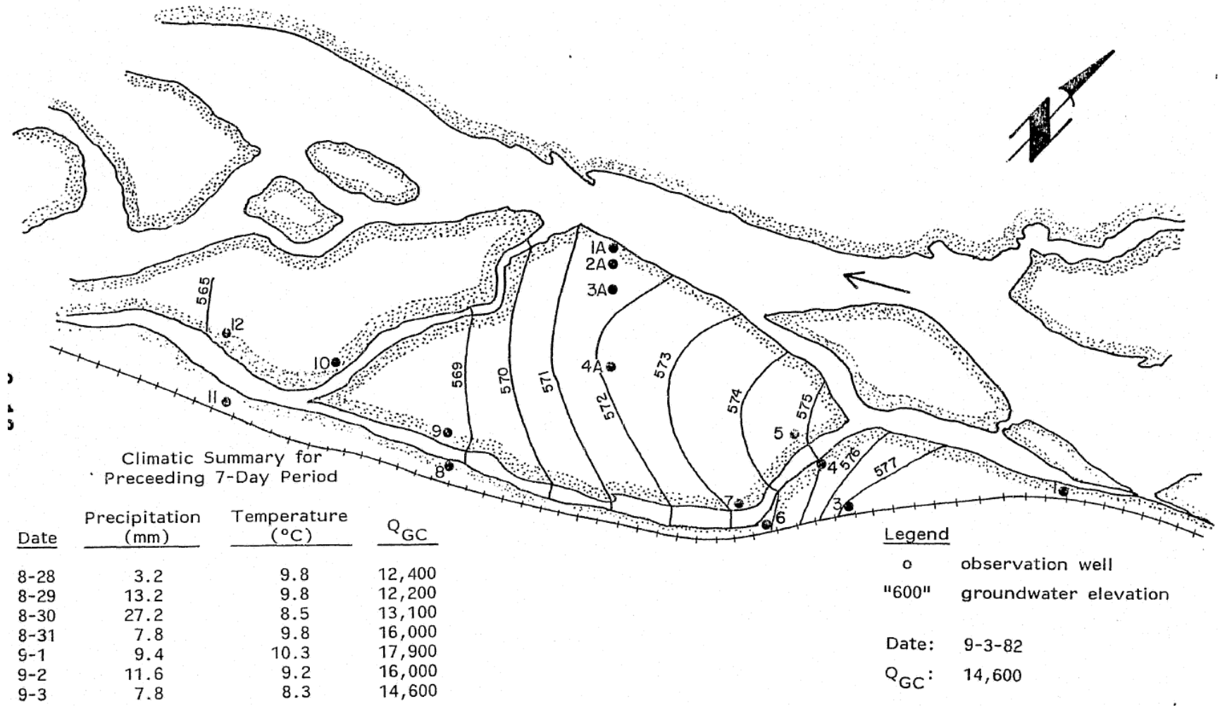
Figure 8. Example groundwater contour map for Slough 8A, from R&M Consultants, (1982).
