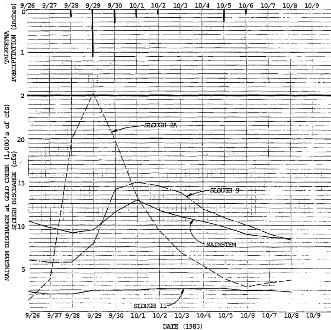
Figure 13. Response of Susitna River and Sloughs 8A, 9, and 11 to a September 1983 Storm, from R&M Consultants and Woodward-Clyde Consultants (1985).
