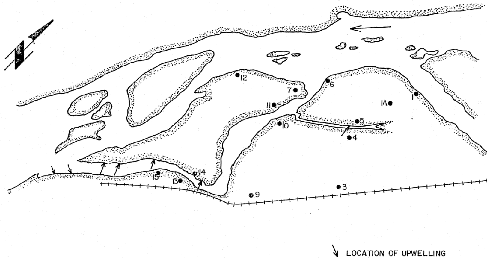
Figure 4. Observed locations of groundwater upwelling in Slough 9 in the Middle Susitna River Segment of the Susitna River, from R&M Consultants, (1982). Slough 9B is located between wells 4 and 5.
