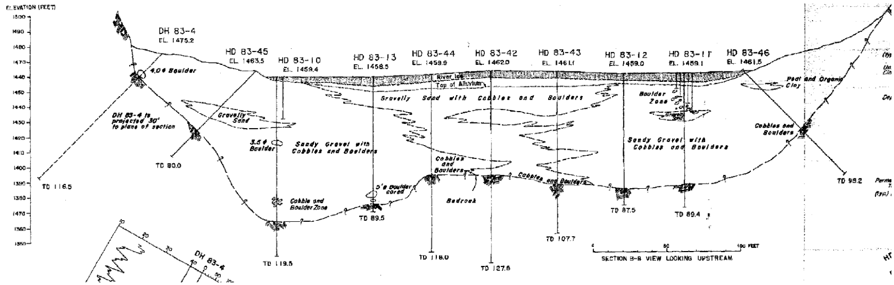
Figure 7. Geologic Cross-section of the Susitna River Channel at the Watana Dam Site, from Harza-Ebasco (1983).
