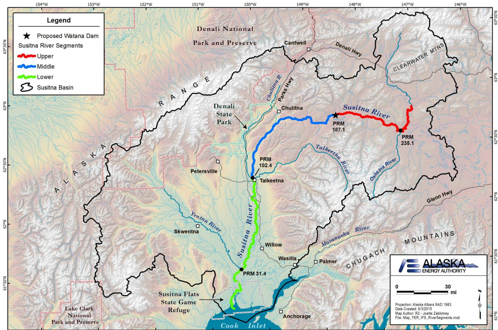
Figure 1. Susitna Watershed basin boundaries, showing the Project designation of Upper, Middle, and Lower Susitna River segments.
