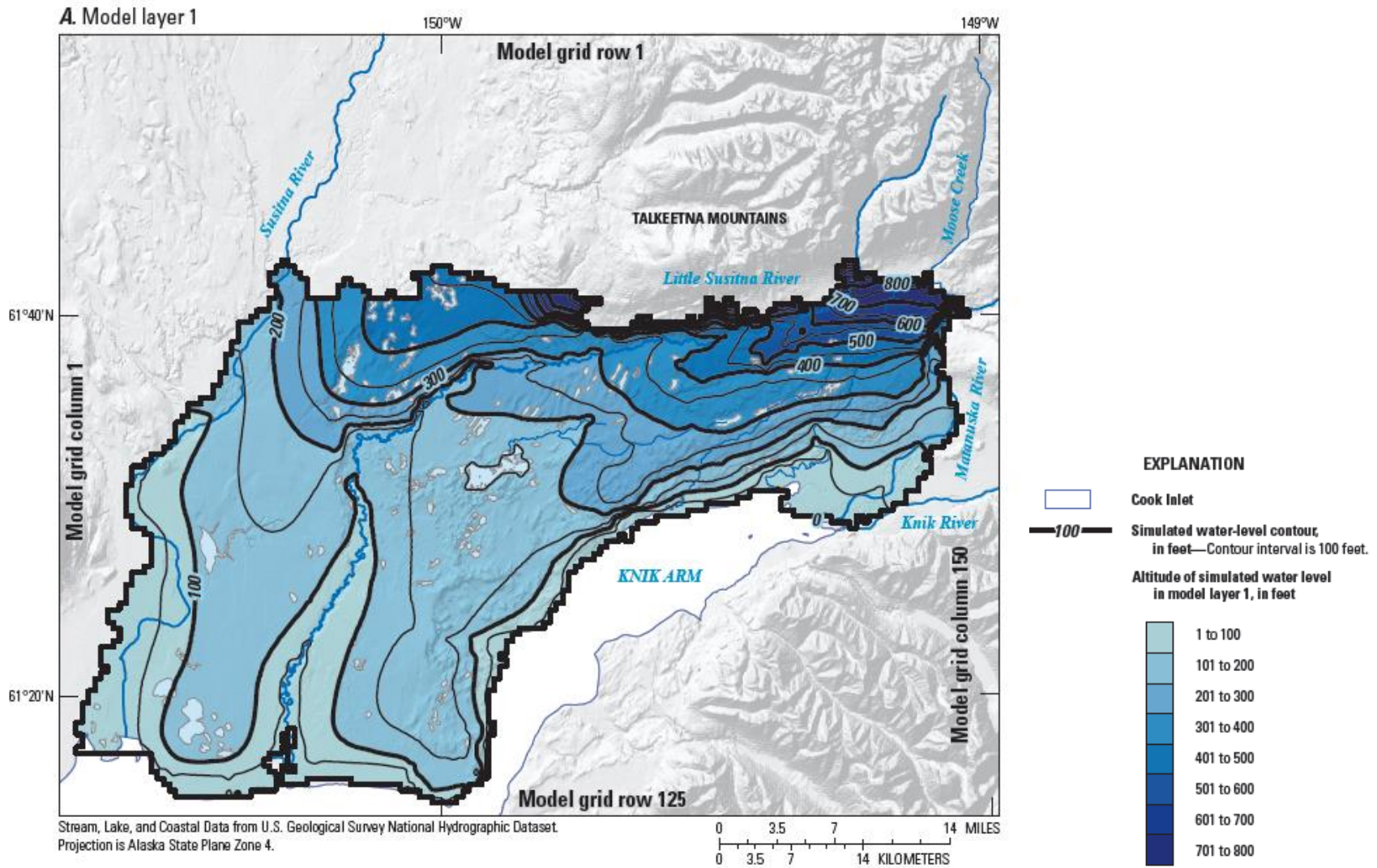
Figure 6. Simulated water levels for shallow sediments in the Matanuska-Susitna Valley, Alaska, from USGS (2013).
