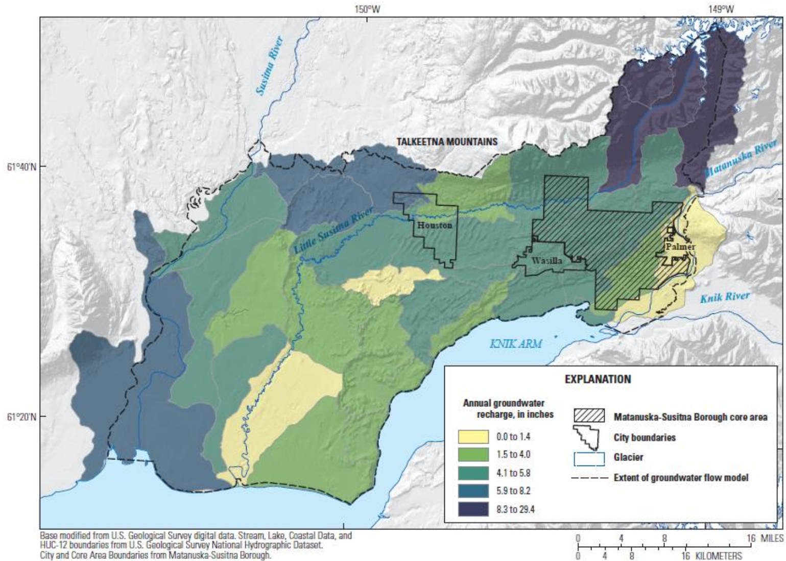
Figure 5. Groundwater recharge for part of the Lower Susitna River Segment, from USGS (2013).
